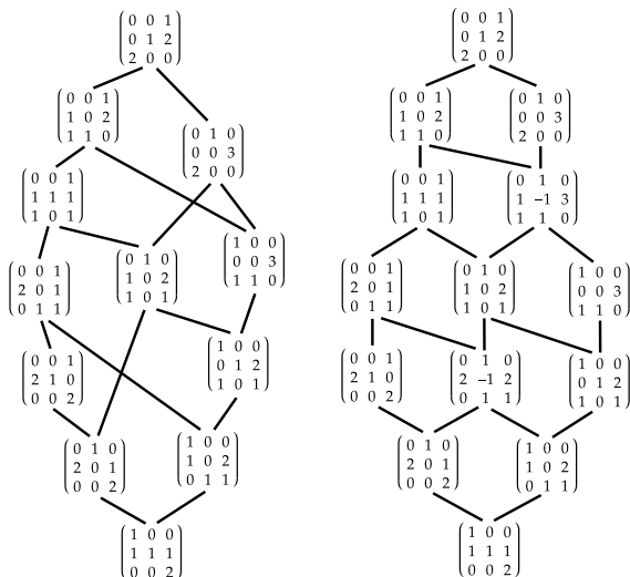
Figure: The Bruhat order on G_{132} \setminus G_6 / G_{213} and its completion.
