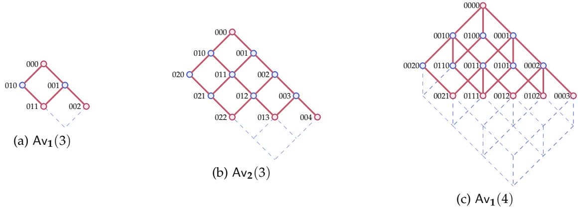
Figure 1: Hasse diagrams of some \delta -avalanche posets.
