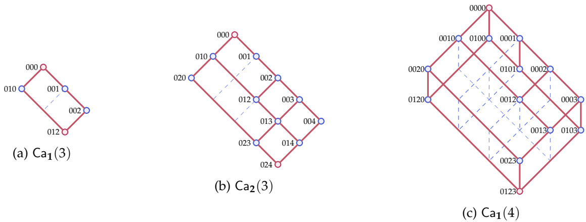
Figure 3: Hasse diagrams of some \delta -canyon posets.
