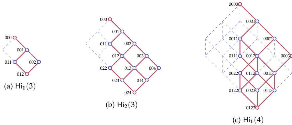
Figure 2: Hasse diagrams of some \delta -hill posets.
