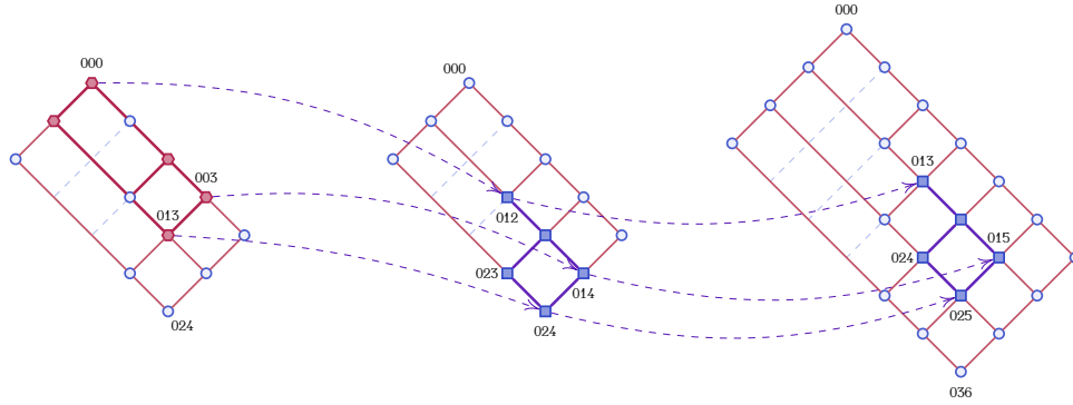
FIGURE 11. From the top to bottom and left to right, here are the posets \text{Ca}_2(3) , \text{Ca}_2(3) , and \text{Ca}_3(3) . The two last posets contain \mathcal{G}(\text{Hi}_1)(3) as subposets. There is a poset morphism between the output-wings of the first one and the input-wings of the second one.
