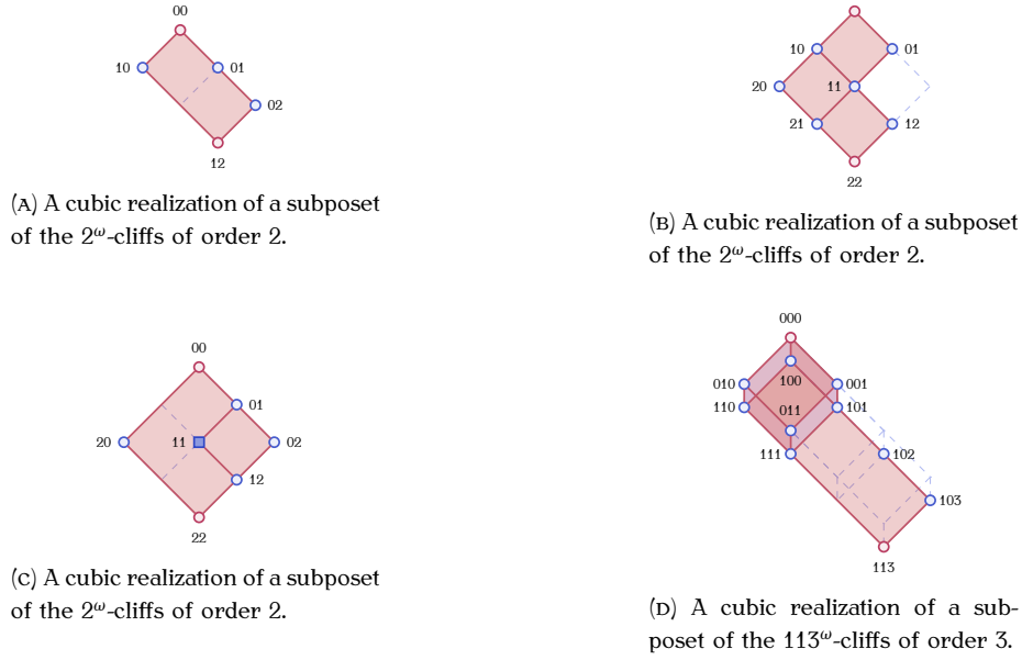
FIGURE 3. Some cubic realizations of straight subposets of posets of \delta -cliffs for certain range maps \delta .
