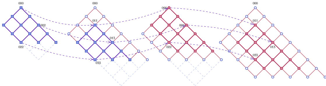
FIGURE 5. From the top to bottom and left to right, here are the posets \text{Av}_2(3) , \text{Av}_3(3) , \text{Av}_3(3) , and \text{Av}_4(3) . All these posets contain \text{Av}_2(3) as subposet by restricting on input-wings, output-wings, or butterflies.
