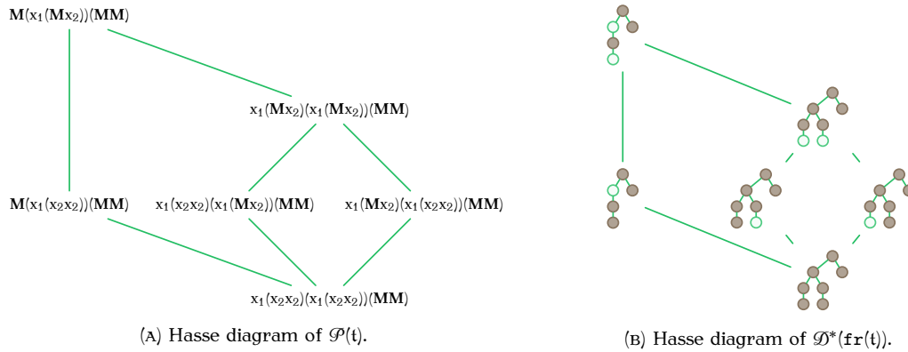
FIGURE 4. A maximal interval of the Mockingbird poset from the term t := \mathbf{M}(x_1(\mathbf{M}x_2))(\mathbf{M}\mathbf{M}) and its realization as a maximal interval in the duplicative forest poset.
