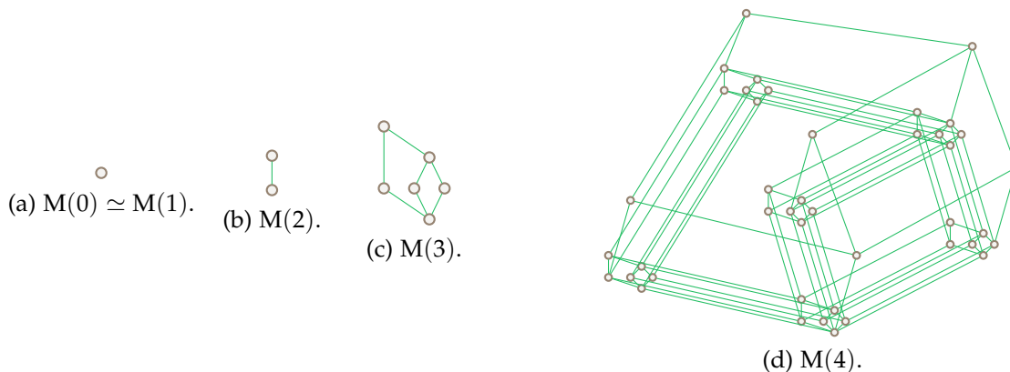
Figure 3: The Hasse diagrams of the Mockingbird lattices M(d) for d \in [4] .
