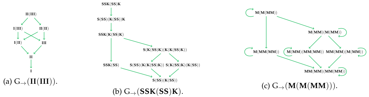
Figure 1: Some subgraphs of rewrite graphs of some CLS.
