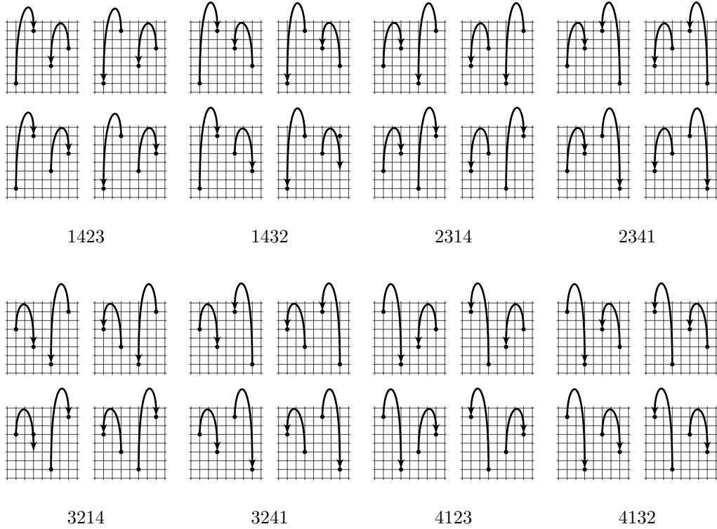
Figure 5: The labeled patterns with consecutive edges avoided by any directed perfect matching on a permutation satisfying Property \mathbf{P}_2 .
