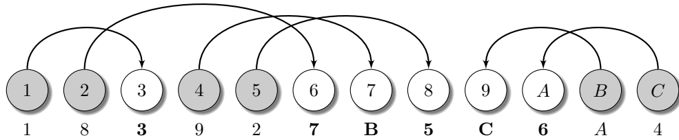
Figure 3: A directed perfect matching \mathcal{M} on the permutation \pi = 183927B5C6A4 satisfying the properties P 1 and P 2 . From \mathcal{M} , it follows that \pi is a square as it appears in the shuffle of 1892A4 and 37B5C6 , both being order-isomorphic to 145263, a square root of \pi .
