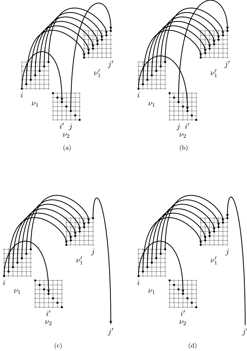
Figure 10: Illustration of Claim 5.12.
