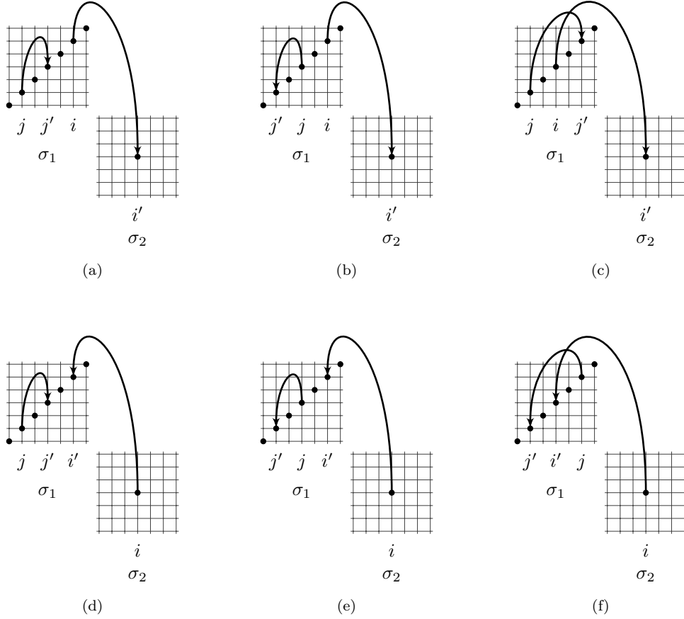
Figure 7: Illustration of Lemma 5.7.
