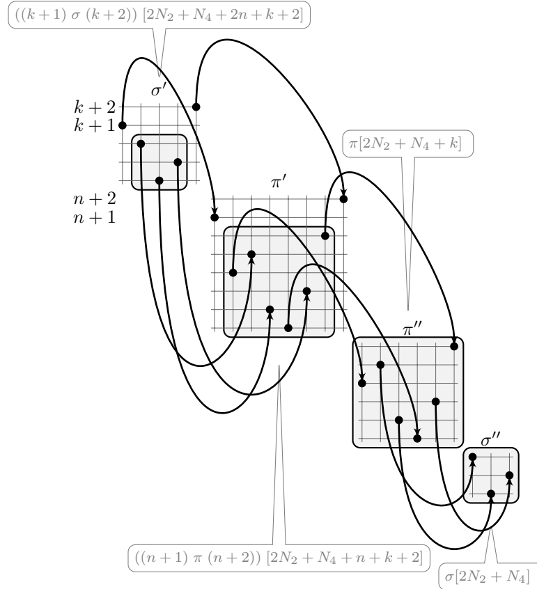
Figure 9: Illustration of the directed perfect matching \mathcal{M} between gadgets \sigma' , \pi' , \pi'' and \sigma'' assuming two input permutation \sigma = 312 and \pi = 4\mathbf{52136} (where a specific occurrence of \sigma in \pi is depicted in bold).
