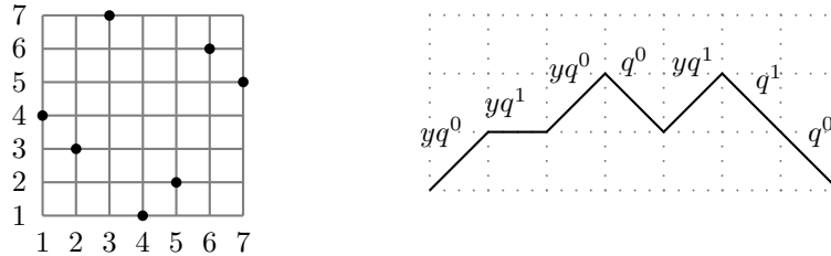
FIGURE 1. Example of the permutation 4371265 and its image under the Françon-Viennot bijection.
