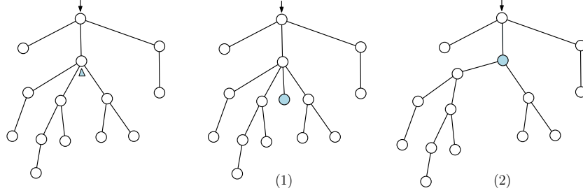
FIGURE 4. Rémy’s procedure gives two ways to obtain a plane tree with n edges and a marked vertex v from a plane tree with n - 1 edges and a marked corner: (1) in the first way (replacing the marked corner by a leg) v is a leaf, (2) in the second way (stretching an edge to carry the subtree on the left of the marked corner) v is a non-leaf.
