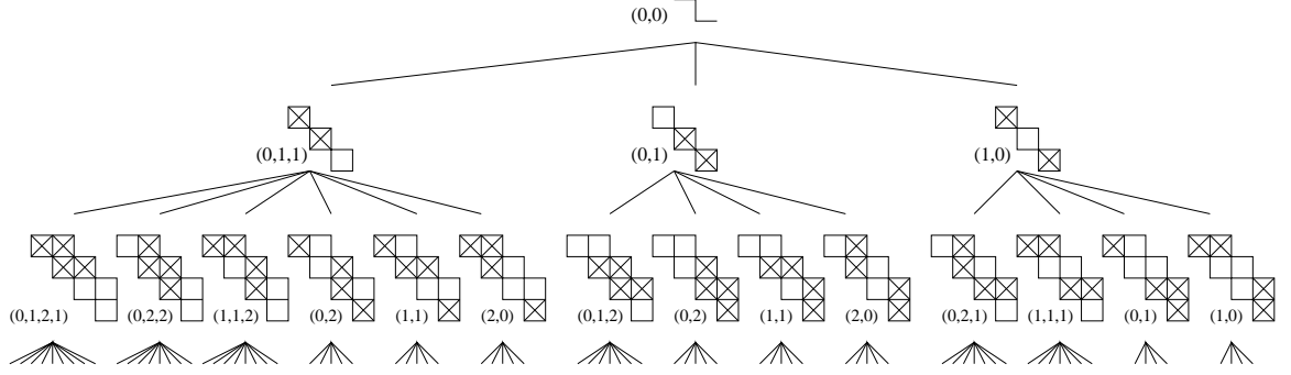
FIGURE 6. The first levels of the generating tree for 2-triangulations.
