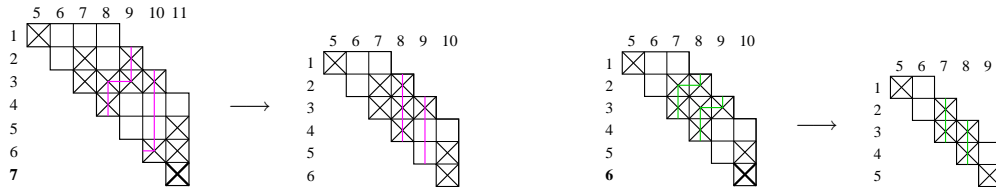
FIGURE 8. The construction of the parent (left) and the grandparent (right) of a 3-triangulation.
