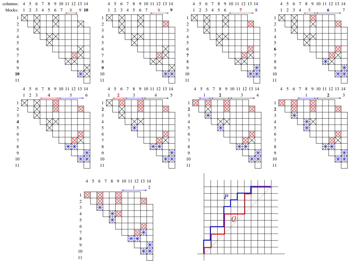
FIGURE 3. An example of the coloring algorithm. The last picture shows the pair \Psi(T) = (P, Q) , where T is the 2-triangulation from Figure 2.
