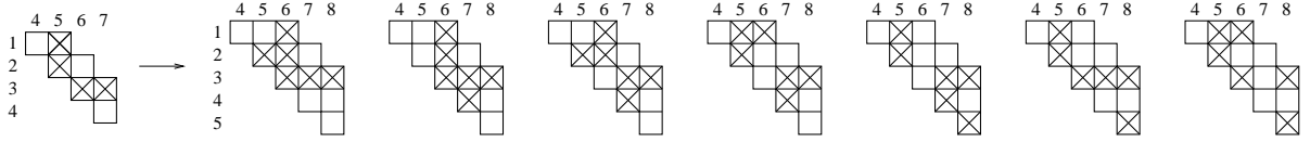
FIGURE 5. A 2-triangulation of an heptagon and its 7 children in the generating tree.
