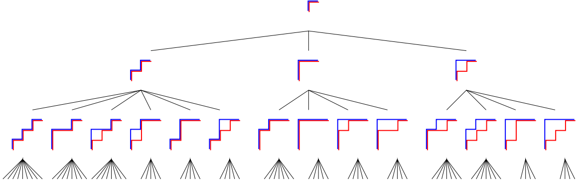
FIGURE 7. The first levels of the generating tree for 2-triangulations.
