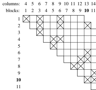
FIGURE 2. A 2-triangulation of a 14-gon, with r = 10 .
