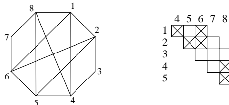
FIGURE 1. A 2-triangulation of an octagon and its representation as a subset of \Lambda_8 .
