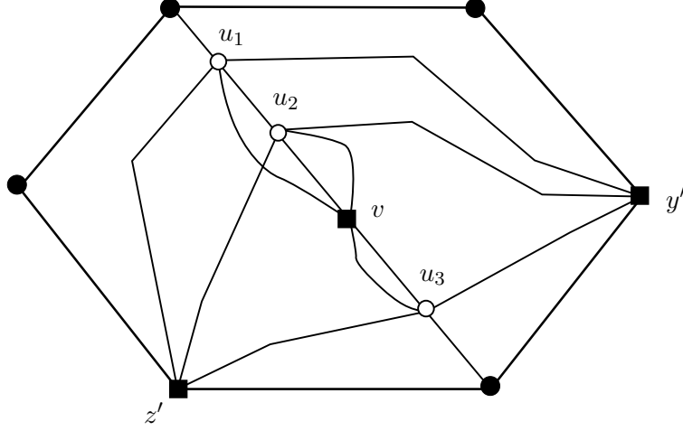
Figure 12: An inactive vertex leads to a K_{3,3} subdivision.
