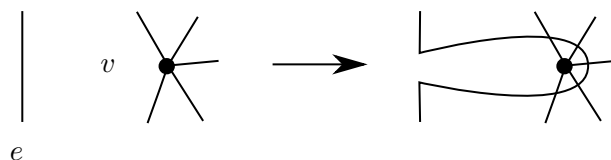
Figure 10: A finger move for a pair p = (e, v) .
