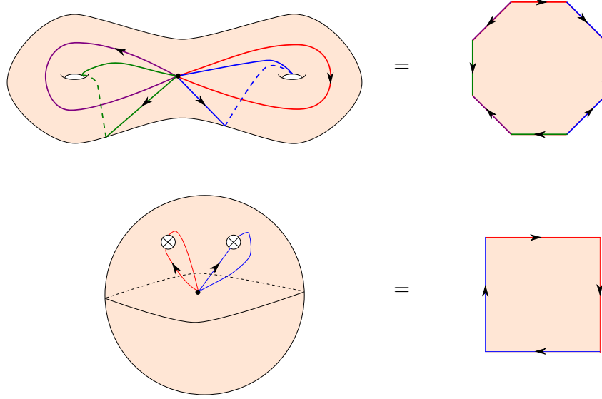
Figure 20: Polygonal schemata of the orientable and non-orientable surfaces. In the non-orientable cases, X denotes a disk on which a Möbius band has been glued.
