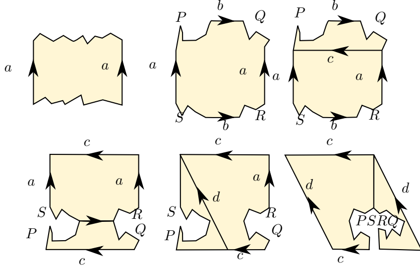
Figure 22: From aPbQ\bar{a}R\bar{b}S to cd\bar{c}d\bar{P}SRQ .
