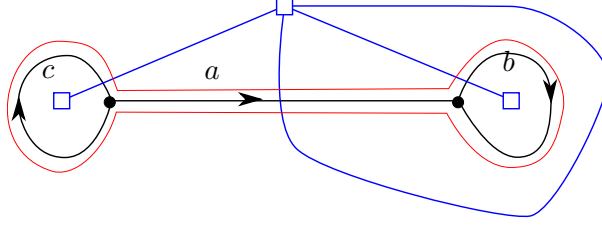
Figure 24: A graph and its dual. The walk ab\bar{a}c is definitely not a cycle in the primal graph, but when we look at it in the cross-metric perspective and push it a bit, it is a nice simple closed curve (in red).
