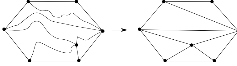
Figure 11: The Tutte magic
