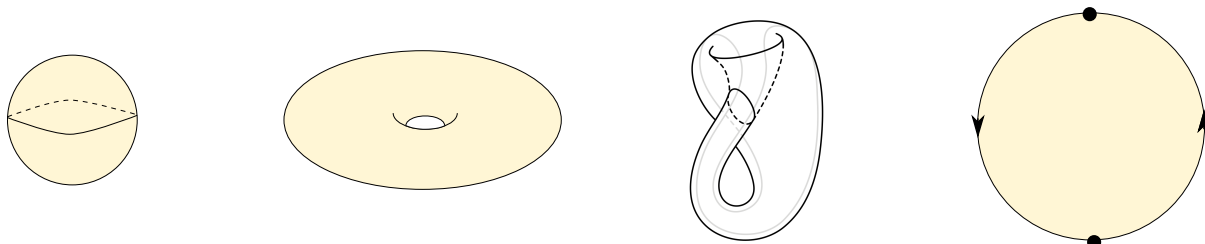
Figure 18: A sphere, a torus, a Klein bottle, and a projective plane (in the last one, the right boundary is identified to the left boundary in the direction indicated by the arrow).
