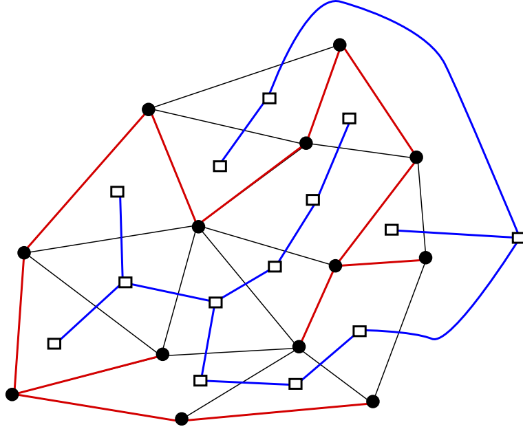
Figure 13: A spanning tree and the spanning co-tree. These are sometimes called interdigating tree.
