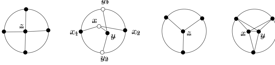
Figure 9: The two cases to find subdivisions of forbidden graphs.
