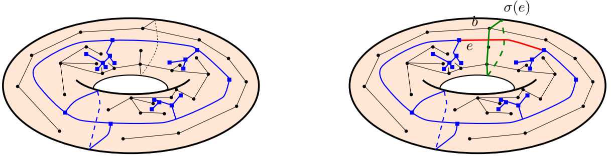
Figure 25: A shortest path tree, in black, defining a cut locus (in blue). Cutting the surface along the cut locus yields a disk. On the right, an edge of the cut locus corresponds to loop \sigma(e) going through the basepoint b .
