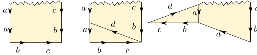
Figure 23: From aabc\bar{b}\bar{c} to \bar{d}\bar{c}\bar{b}\bar{d}\bar{b}\bar{c} .
