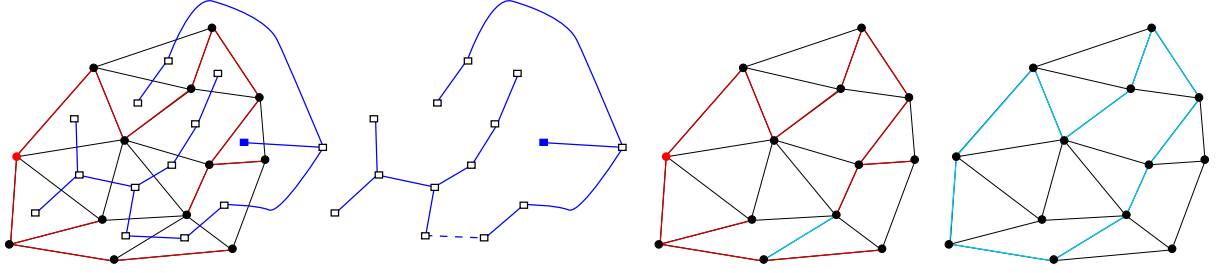
Figure 14: An edge separating the dual co-tree into balanced parts induces a balanced separator in the primal graph.
