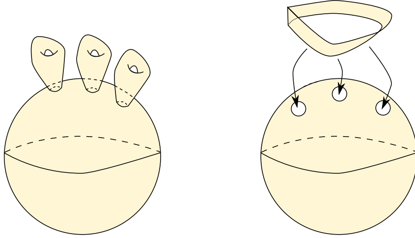
Figure 19: Attaching handles or Möbius bands to a sphere.
