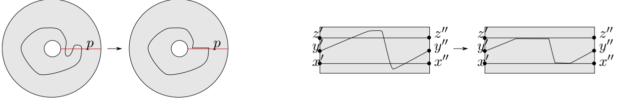
Figure 17: The two shortcutting arguments of Lemma 2.12 and Lemma 2.13.
