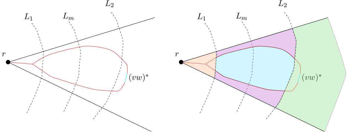
Figure 14: An edge separating the dual co-tree into balanced parts induces a balanced separator in the primal graph.
