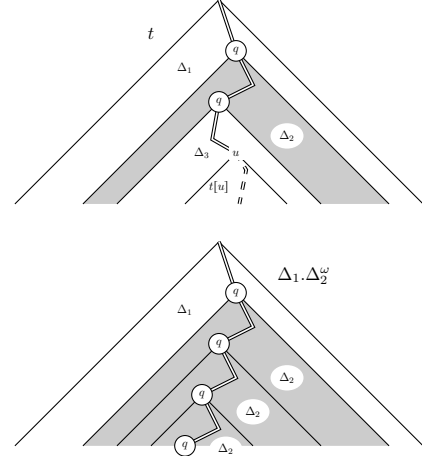
Figure 1. Pumping Lemma
