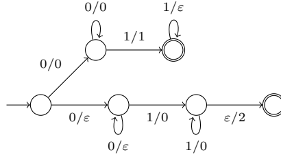
Figure 3. A transducer for the relation from Example 9.
