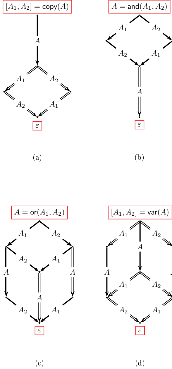
FIG. 14. Abstract representations of the blocks copy , and , or , and var , obtained from each behavior graph (Figures 10, 11, 12, and 13) by contracting arcs corresponding to internal triples, and keeping only the arcs corresponding to variables. We see, for each block, which output variables can be activated, depending on which variables have been activated.
