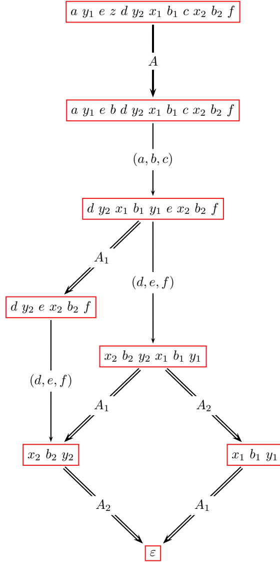
FIG. 10. Behavior graph of the block [A_1, A_2] = \text{copy}(A) . A thick (resp., double) arc corresponds to the 3DT-step \xrightarrow{(x, y, z)} for an input (resp., output) variable [(a, b, c), (x, y, z)] .
