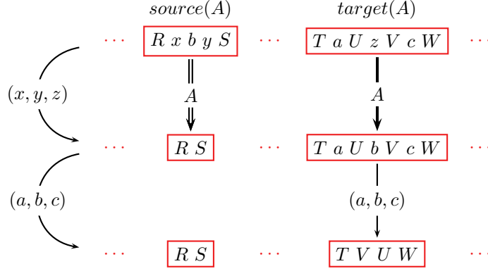
FIG. 9. The activation of a variable A = [(a, b, c), (x, y, z)] is written with a double arc in the behavior graph of the source block of A and with a thick arc in the behavior graph of its target block. It can be followed by the 3DT-step \xrightarrow{(a, b, c)} , impacting only the target block of A . Dot symbols ( \cdot ) are omitted. We denote by R, S, T, U, V, W some factors of the source and target blocks of A : the consequence of activating A is to allow U and V to be swapped in \text{target}(A) .
