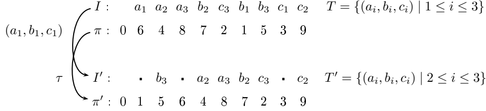
FIG. 6. Illustration of Lemma 7: since I \sim \pi and I \xrightarrow{(a_1, b_1, c_1)} I' , it follows that I' \sim \pi' = \pi \circ \tau , where \tau = \tau[a_1, b_1, c_1, \psi] .
