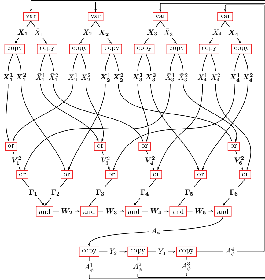
FIG. 16. Schematic diagram of the blocks defining I_\phi for \phi = (x_1 \vee x_2 \vee \neg x_3) \wedge (x_1 \vee \neg x_2) \wedge (\neg x_1 \vee x_2 \vee \neg x_4) \wedge (\neg x_1 \vee x_3 \vee x_4) \wedge (x_3 \vee \neg x_4) \wedge (\neg x_2 \vee \neg x_3 \vee x_4) . For each variable, we draw an arc between its source and target block. Note that \phi is satisfiable (e.g., with the assignment x_1 = x_3 = \text{true} and x_2 = x_4 = \text{false} ). A set of variables that can be activated before A_\phi is in bold; they correspond to the terms being true in \phi for the assignment x_1 = x_3 = \text{true} and x_2 = x_4 = \text{false} .
