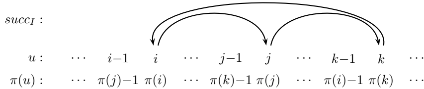
FIG. 5. Illustration of the equivalence I \sim \pi on three integers (i, j, k) such that j = \text{succ}_I(i) and k = \text{succ}_I(j) . It can be checked that \pi(v) = \pi(u - 1) + 1 for any (u, v) \in \{(i, j), (j, k), (k, i)\} .
