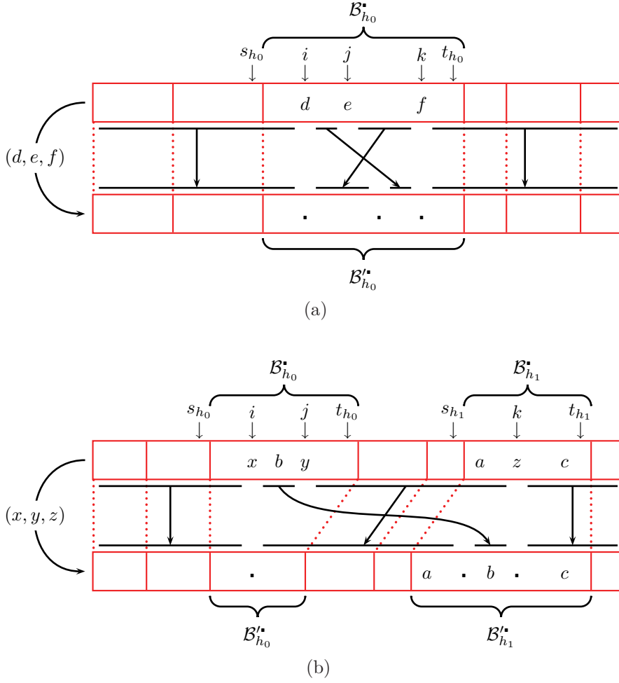
FIG. 8. Effects of a 3DT-step \xrightarrow{(d, e, f)} on an l -block decomposition if (a) (d, e, f) is an internal triple, or (b) there exists a variable A = [(a, b, c), (x, y, z)] such that (d, e, f) = (x, y, z) . Both figures are in fact derived from Figure 3 in the context of an l -block decomposition.
