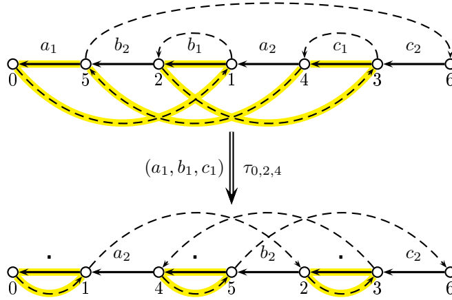
FIG. 7. The 3DT-instance a_1 \ b_2 \ b_1 \ a_2 \ c_1 \ c_2 seen on the corresponding cycle graph, i.e., the cycle graph of permutation (0, 5, 2, 1, 4, 3, 6) . The ordered triple (a_1, b_1, c_1) corresponds to the overlined oriented 3-cycle, and following the 3DT-step, removing this triple corresponds to breaking the cycle into 1-cycles.
