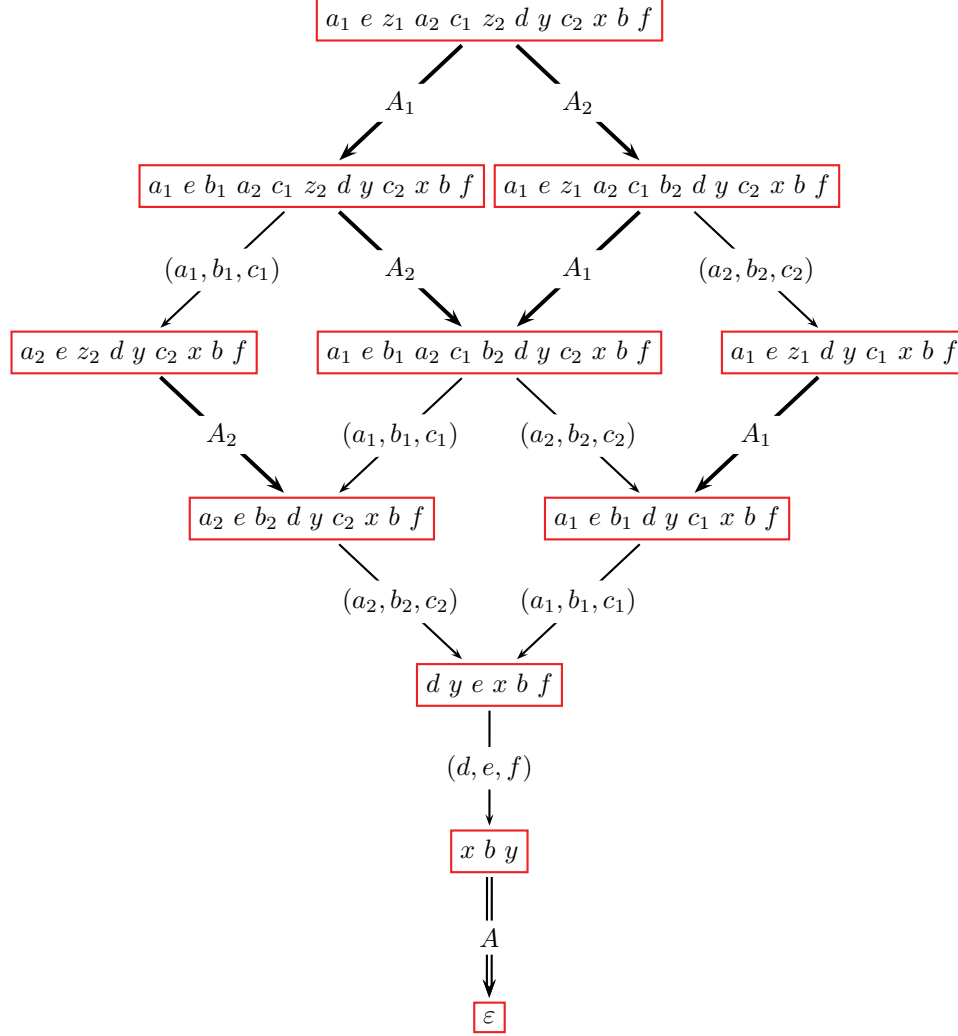
FIG. 11. Behavior graph of the block A = \text{and}(A_1, A_2) .
