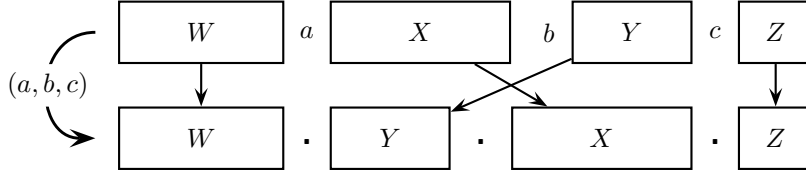
FIG. 3. The 3DT-step \xrightarrow{(a,b,c)} has two effects, shown here on the word representation of a 3DT-instance: the triple (a,b,c) is deleted (and replaced by dots in this word representation), and the factors X and Y are swapped.
