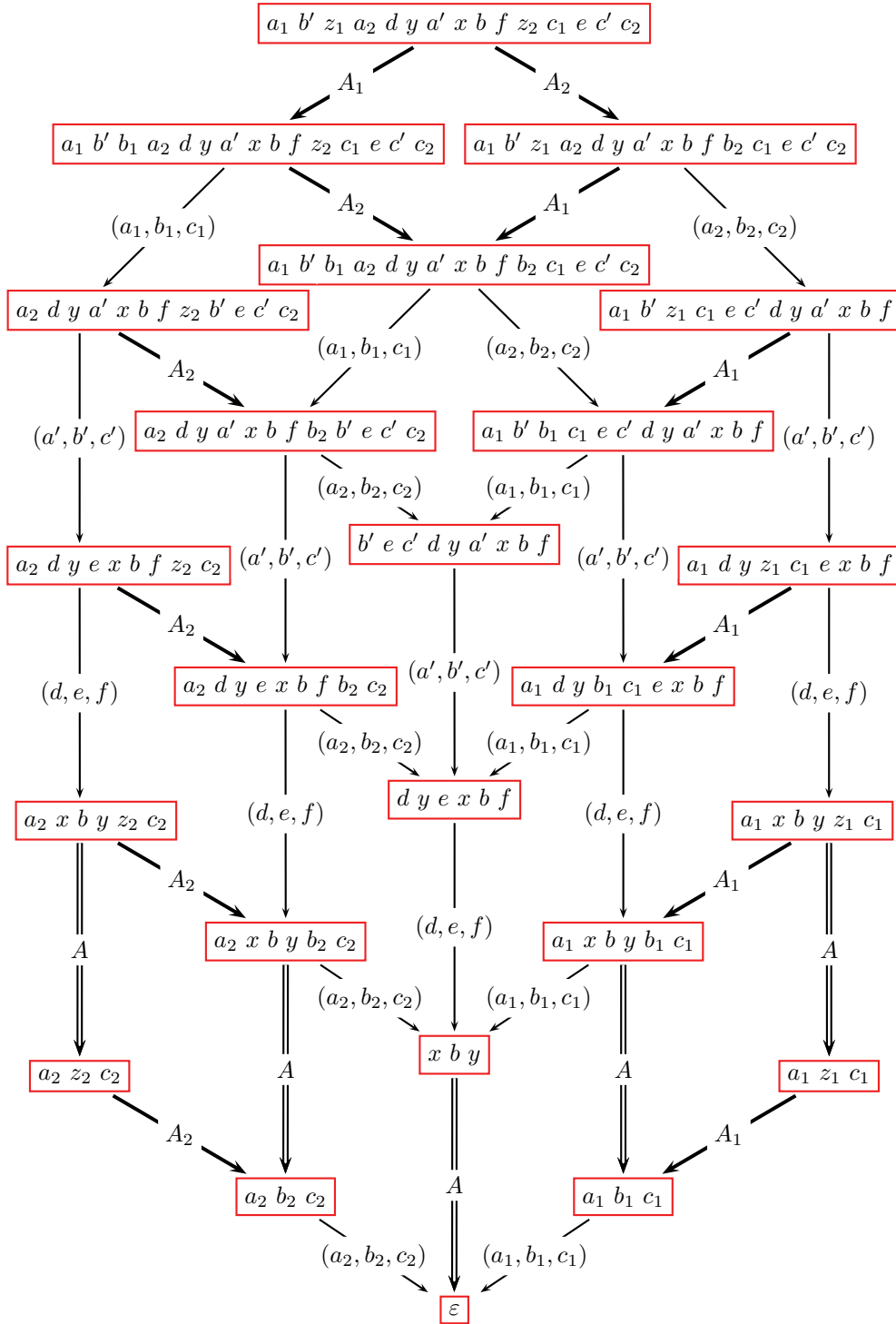
FIG. 12. Behavior graph of the block A = \text{or}(A_1, A_2) .
