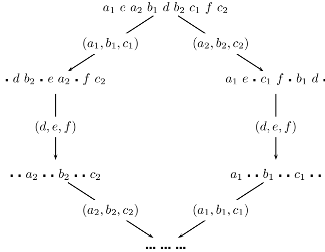
FIG. 4. Possible 3DT-steps from the instance I defined by the word a_1 e a_2 b_1 d b_2 c_1 f c_2 and the set of triples T = \{(a_1, b_1, c_1), (a_2, b_2, c_2), (d, e, f)\} . We can see that there is a path from I to \varepsilon ; hence I is 3DT-collapsible. Note that both (a_1, b_1, c_1) and (a_2, b_2, c_2) are well-ordered in the initial instance; each one loses this property after applying the 3DT-step associated to the other and becomes well-ordered again after applying the 3DT-step associated to (d, e, f) .
