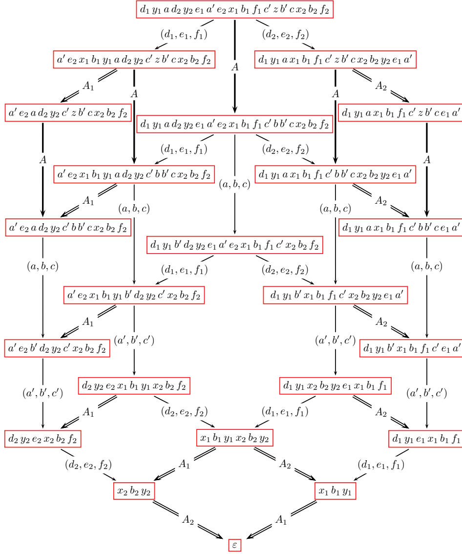
FIG. 13. Behavior graph of the block [A_1, A_2] = \text{var}(A) .
